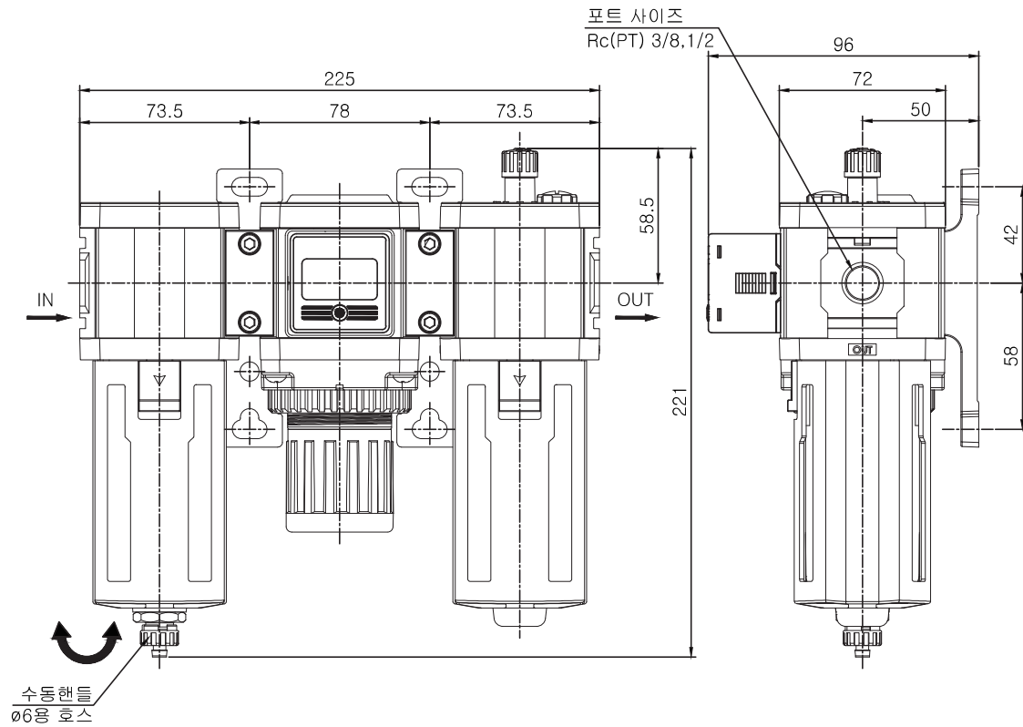
Combination Type (Filter+Regulator+Lubricator)
